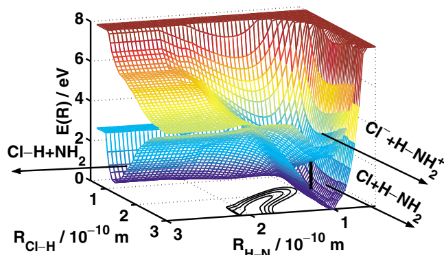
FIG. 1 (color online). Adiabatic potential energy surfaces for the ground (neutral) and the lowest charge transfer state of the Cl \cdots NH 3 complex. The contours represent the energy gap in the avoided crossing region. The vertical bar indicates the center of the Franck-Condon region for vertical transition from the anionic precursor.
