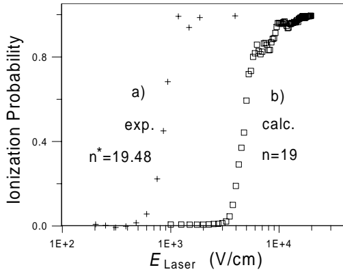
Fig. 1. Experimental (a) and simulated (b) ionization onset curves as a function of FIR laser field strength.
