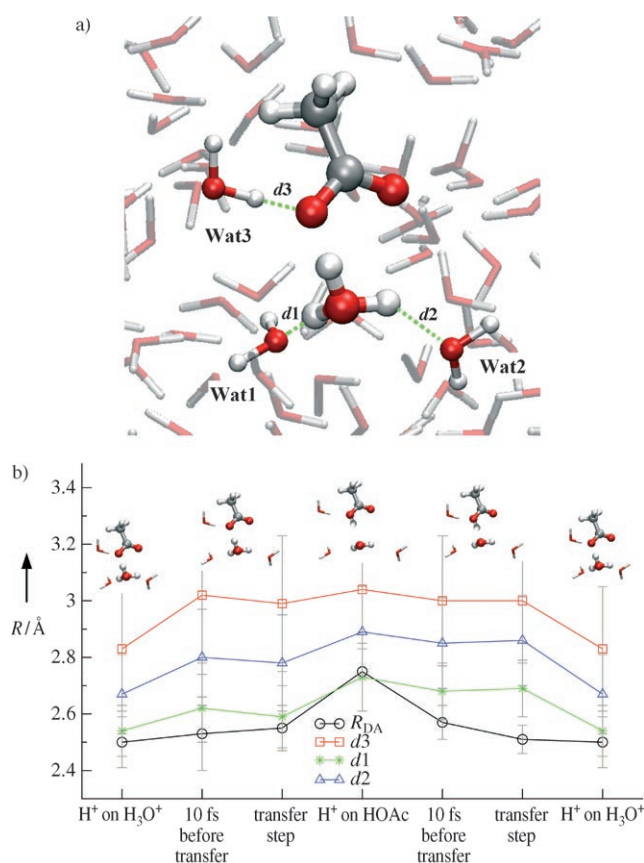
Figure 3. a) A snapshot of a typical transfer scenario observed during the simulation. The donor ( H_3O^+ ) and the acceptor (AcOH) as well as the three closest water molecules are shown using the “atom and bond” representation. O red, H white. The green dashed lines represent possible hydrogen bonds. b) Evolution of the distances R_{DA} and d1 – d3 . R_{DA} : O_\delta – OW(H_3O^+) , d1 : OW(H_3O^+) – OW1 , d2 : OW(H_3O^+) – OW2 , d3 : O_\delta – OW3 . ■■Zuordnung ok?■■■
