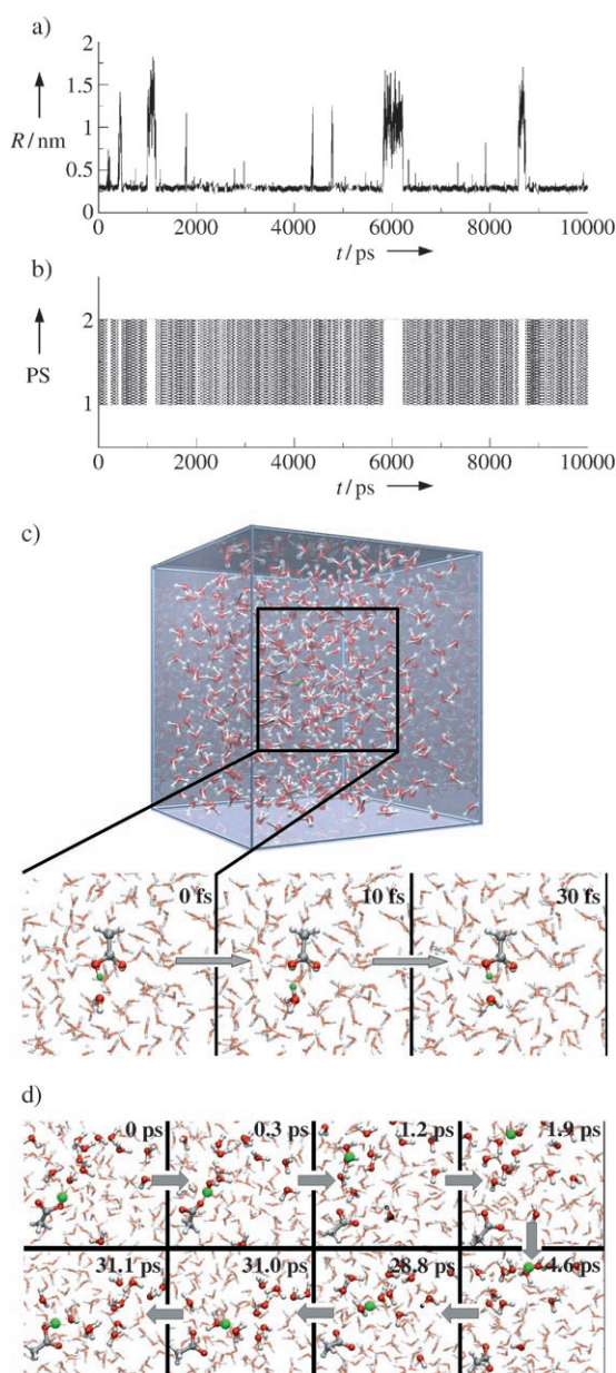
Figure 1. a) Time evolution of the distance ( R ) between the O_{\delta} atom of acetic acid and the O atom of H_3O^+ . b) Time evolution of the protonation states (PS) of the system: 1 denotes the state in which the proton is located on the acetic acid, 2 denotes the state in which the proton is bound to H_3O^+ . c) Snapshots of a “fast-swapping” phase (the simulation box is shown at the top and the donor–acceptor pair is enlarged). d) Snapshots of a typical traveling phase lasting 31 ps and involving 16 different water molecules. Only the first four and the last three transfer steps and the molecules involved are shown; oxygen atoms are red, and protons that are transferred are green.
