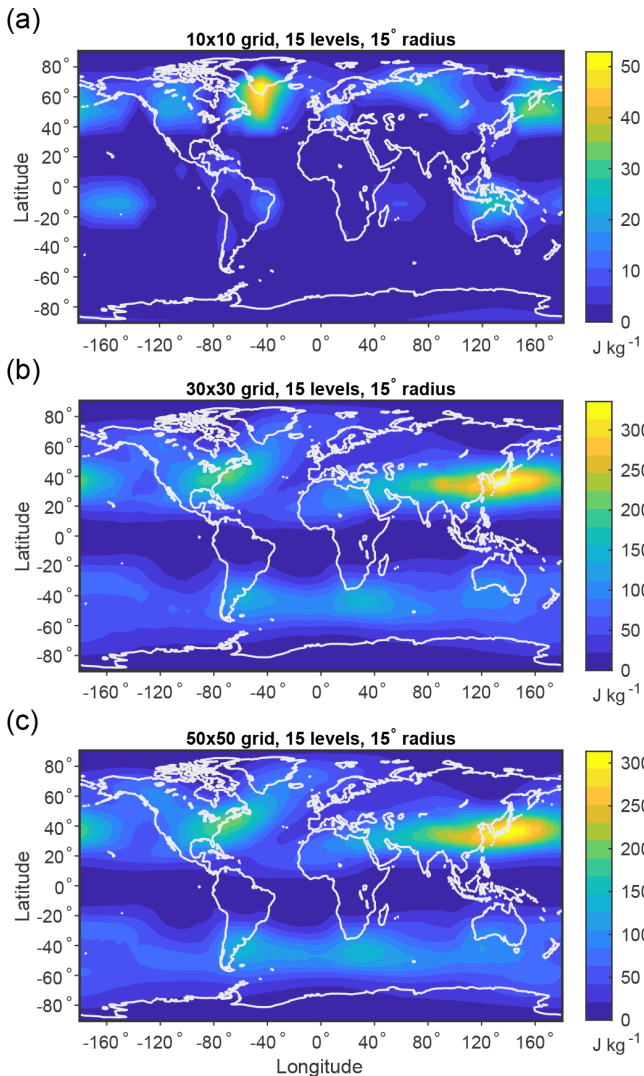
Figure B1. Local MAPE based on the DJF climatological mean over 1979–2018 for grids of varying horizontal resolution: (a) 200 surface grid cells (a 10 × 10 grid in each hemisphere), (b) 1800 surface grid cells (a 30 × 30 grid in each hemisphere), and (c) 5000 surface grid cells (a 50 × 50 grid in each hemisphere). All results shown in this figure use 15 pressure levels and subdomains of geodesic radius of 15° (1670 km).
