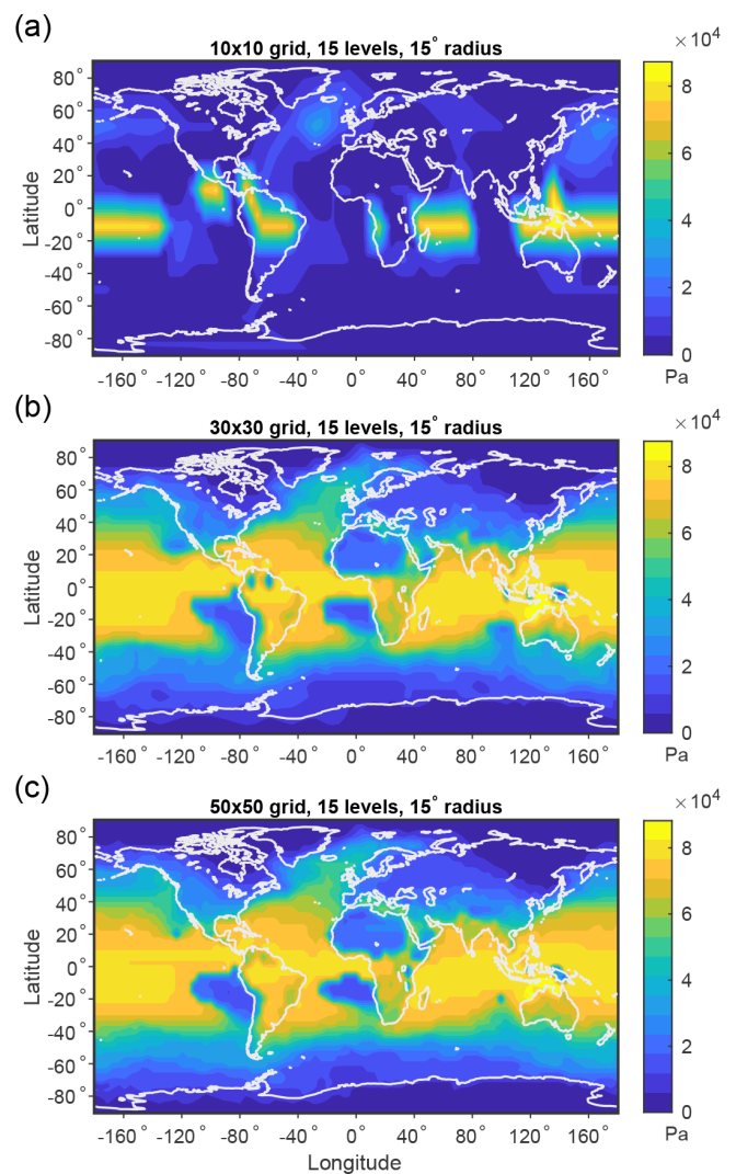
Figure B2. Maximum potential ascent in local MAPE based on the DJF climatological mean over 1979–2018 for grids of varying horizontal resolution: (a) 200 surface grid cells (a 10 × 10 grid in each hemisphere), (b) 1800 surface grid cells (a 30 × 30 grid in each hemisphere), and (c) 5000 surface grid cells (a 50 × 50 grid in each hemisphere). All results shown in this figure use 15 pressure levels and subdomains of geodesic radius of 15° (1670 km).
