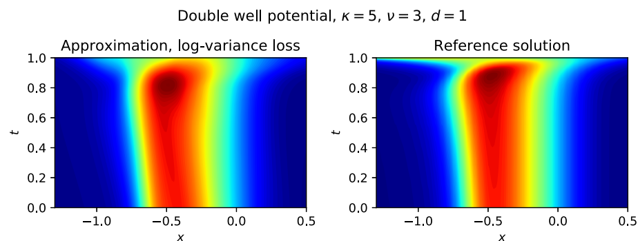
Fig. 11 Approximation and reference solution for the double well control problem in d = 1
