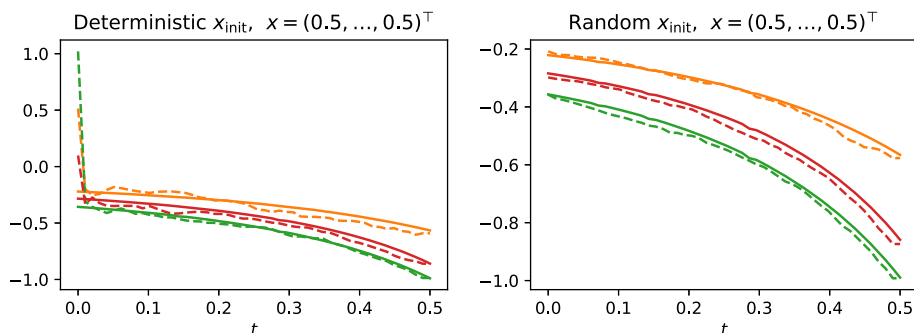
Fig. 7 Approximation and reference solution of the optimal control with either deterministic or random initialisations of x_{\text{init}} . Three components of u and u_{\text{ref}}^* are plotted
