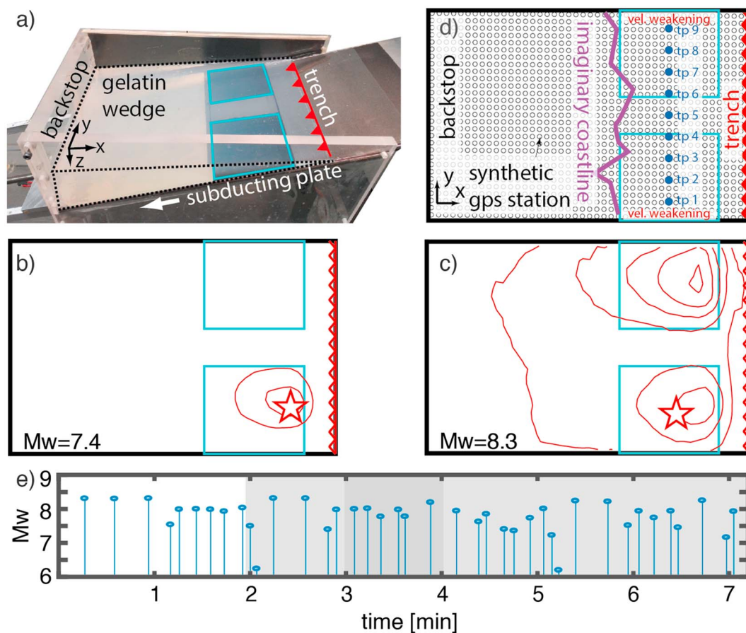
Figure 1. Analog model of megathrust earthquakes. (a) Oblique view of the experimental setup. Cyan rectangles highlight the two velocity weakening patches. The analog model produces spontaneous ruptures that involve either (b) one or (c) both velocity weakening zones. Ruptures are characterized in terms of apparent slip (i.e., coseismic surface displacement; red contour with interval of 0.15 mm). White/red stars in (b) and (c) represent the epicenters. (d) Experimental monitoring is performed with a video camera from top view (orthogonal to the x - y plane); image analysis allows dense resolution of the velocity field (white points) also above the offshore seismogenic zone. The nine blue points highlight target stations used for the machine learning analysis. (e) Time series of analog earthquakes magnitude. The light and dark gray shading highlight the fraction of the experiment shown in Figures 3a and 3b and the zoom of Figure 3c, respectively.
