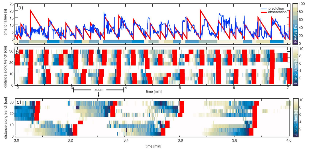
Figure 3. Machine learning results. (a) TTF versus experimental time. The red and blue time series refer to observation and prediction, respectively. The color-coded horizontal line highlights the performances of the prediction cycle by cycle quantified by means of relative root-mean-square error (RRMSE). Dark blue RRMSE colors highlight cycles with a good fit. (b) Space–time evolution of the predicted time to failure calculated for the nine target points. The blue shading highlights the prediction of an upcoming event at a given location. The red squares indicate the spatiotemporal distribution of observed analog earthquakes (width of red squares not scaling with time). (c) One-minute long zoom of (b). Synchronous existence of low time to failure values for several target points along the margin suggests that a large-magnitude earthquake is impending.
