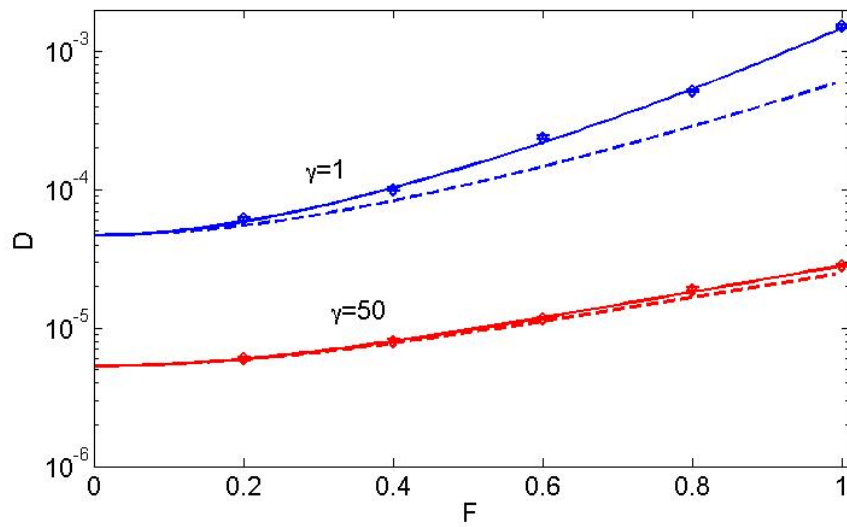
Figure 6: D for \gamma = 1 (blue lines) and \gamma = 50 (red lines). Solid lines: Homogenization formula (16a). Broken lines: Computation of D assuming the Einstein relation (27), with derivative evaluated through centered finite differences of the drift computed from the homogenization formula (15). Parameters of the simulation as in Figure 4.
