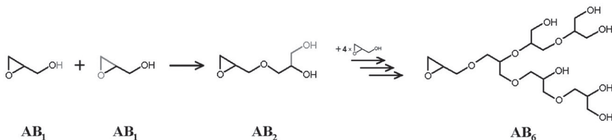
Scheme 2. Ring-opening reaction scheme for two glycidol monomers forming an AB_2 dimer (glycidyl glycerine). By binding more monomers a dendritic polymer AB_n (e.g., n=6 ) is created.
