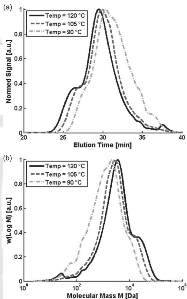
Figure 2. (a) Observed elution time diagram of the final samples (reaction time t=18 h) at different temperatures and (b) molar mass distributions calculated from the elugrams with help of the calibration curve.
