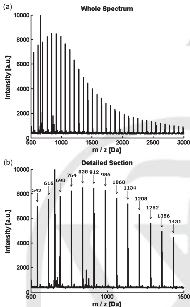
Figure 1. Complete MALDI-TOF mass spectrum (a) for the final sample (reaction time t=18 h) of the experiment at 105^{\circ}\text{C} . A detailed inspection (b) shows a series of distinct peaks that can be associated with polymers of different sizes.
