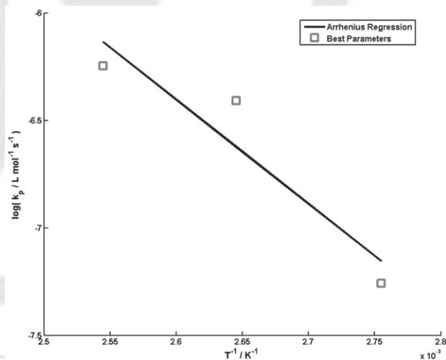
Figure 4. Arrhenius plot for k_p . The markers indicate the optimal values for the three reaction temperatures. The solid line shows the result of the linear regression.
